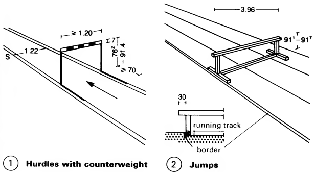
1 Hurdles with counterweight
